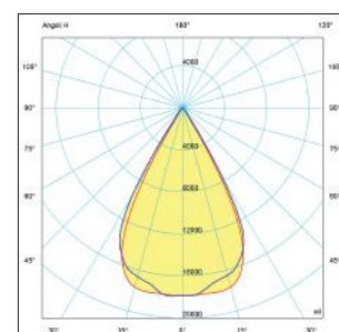
SLED-ME-400200 Luminous flux: 20744 lm
