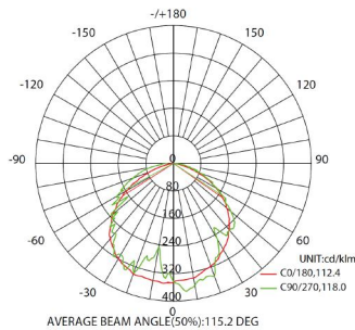
ZNF.22W - 6500K
