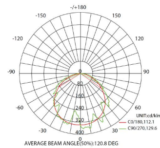
ZNF.66W - 6500K
