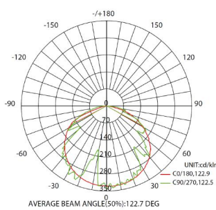
ZNF.44W - 6500K
